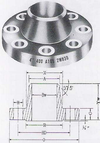
WELDING NECK
