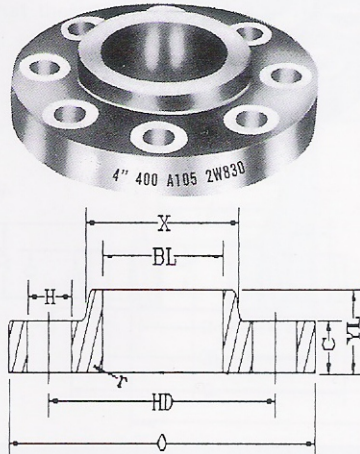
LAP JOINT
