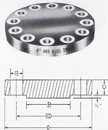
BLIND
