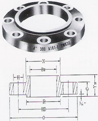
SLIP-ON
