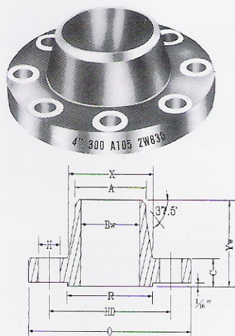
WELDING NECK
