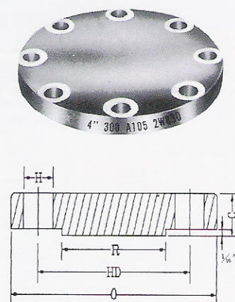
BLIND
