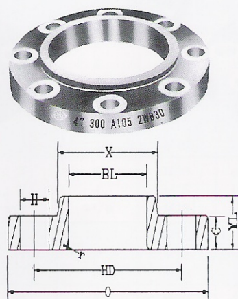
LAP JOINT
