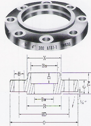
SOCKET WELDING
