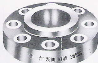
LAP JOINT
