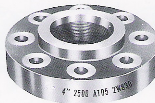
SCREWED
